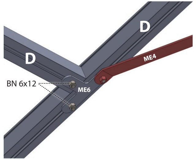
Not used for sizes L = 63.23"; 92.60"
