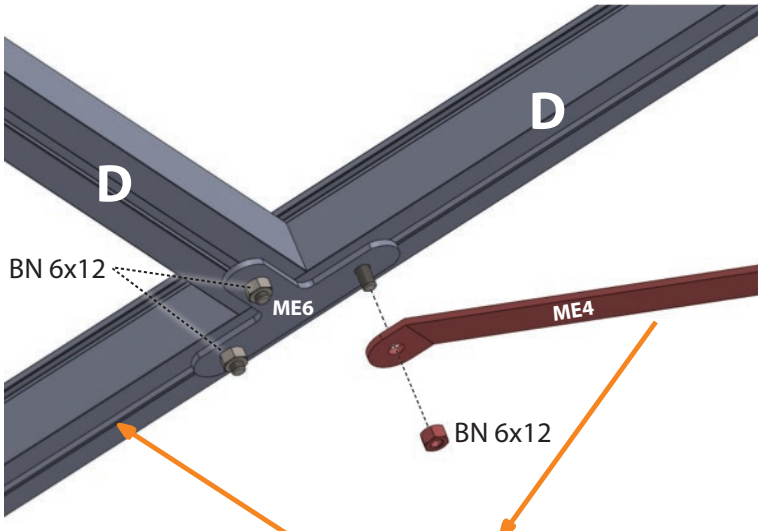
Install ME4 lower with extra screw if your house W=92.56"
