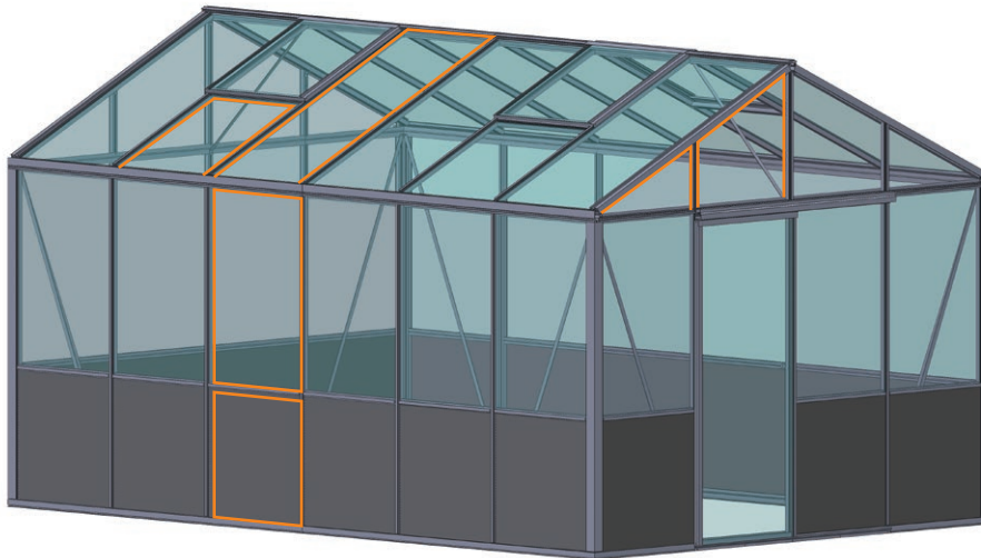
Rubber placement
